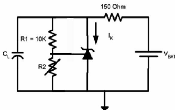
Test Circuit for V_{KA} = 2V, 3V
